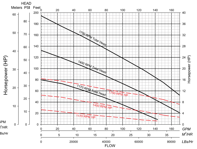
WCB 2085LR - Total Head and Horsepower vs Flow
